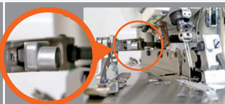
抬压脚安全感应装置 Presser foot lift safety sensor
